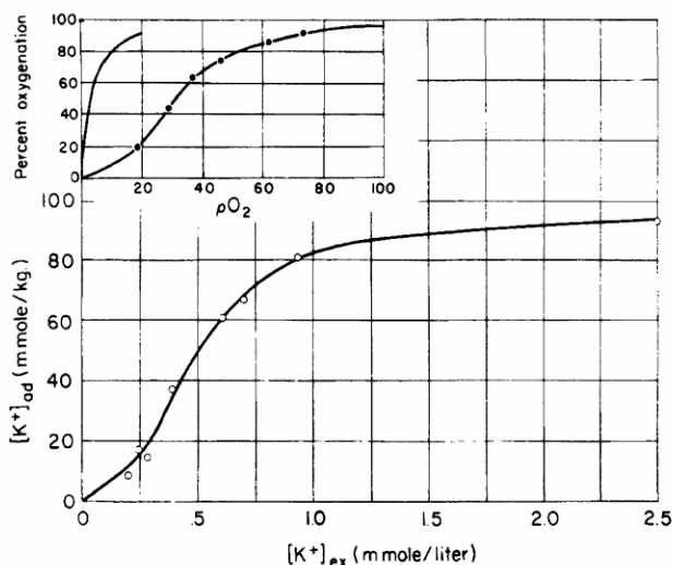
Figure 55. Equilibrium K^+ concentration in frog sartorius muscles at 25^\circ\text{C} in Ringer's solution containing an unvarying high concentration of \text{Na}^+ concentration (100 mM) but varying (low) K^+ concentration (abscissa). The sigmoid profile resembles that of oxygen uptake by human erythrocytes shown in the inset as the line going through or near the filled circles. The solid line to the left in the inset shows oxygen uptake of isolated myoglobin. (Inset from Eastman et al. 440 ) (Ling 439 by permission of Federation Proceedings )
