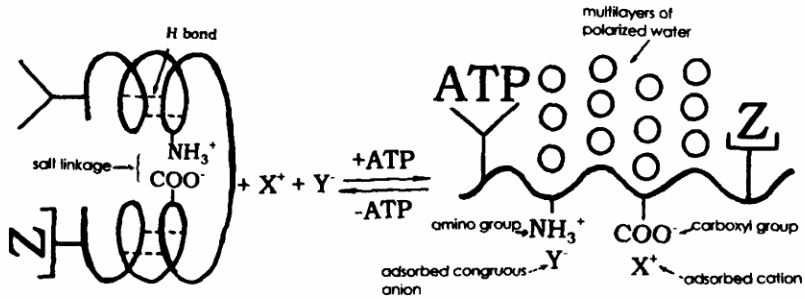
Figure 44. Diagrammatic illustration of how adsorption of the cardinal adsorbent ATP on the ATP-binding cardinal site and of “helpers” including the congruous anions (shown here as “ad- sorbed congruous anion”) and Protein-X (shown as Z) unravels the introverted (folded) secondary structure shown on the left-hand side of the figure. As a result, selective K + adsorption can now take place on the liberated β- and γ-carboxyl groups (shown on the right side of the figure as carboxyl groups) and multilayer water polarization and orientation can now occur on the exposed backbone NHCO groups and the resting living state is thus achieved and maintained. (This figure is the latest modified version of an original (simpler) version first published in 1969 in Reference 173.)
