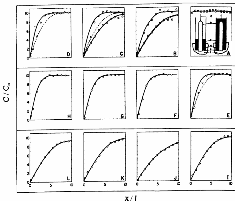
Figure 10. Diffusion profiles of labeled K^+ from surviving (B to H) and dead (I to L) frog sartorius muscles. Ordinate represents concentrations ( C ) of labeled K^+ (A to L) or of tritiated water (in A–C only) as fractions of their respective initial concentration in the muscle ( C_0 ). Abscissa represents the distance x from the cut end of the muscle expressed as a fraction of the total length, l , of the (amputated) muscle. Circles, ^{42}K^+ ; squares, tritiated water. Circles, squares (and lines going through or near most of the circles or squares) at top of A represent respectively ^{42}K and tritiated water concentration along the length of an intact unwashed normal frog sartorius muscle. For more details of EMOC preparation used (shown sketchily here in A), see Figure 7. Solid lines are theoretical diffusion profiles that fit all the points with a single ( D_K t/l^2 ) value (F to L), where D_K is the diffusion coefficient of K^+ , t is the duration of the experiment and l is as defined above, the total length of the (amputated) muscle. In composite figures C to E, each dotted line and the accompanying solid line fit only part of the data points. Muscles in I to L were killed by prior exposure to the metabolic poison, iodoacetate, and were in full rigor before being mounted on the EMOC setup but were kept at their initial normal relaxed lengths at all times. (Ling and Ochsenfeld, 312 with permission from Science copyright 1973. American Association for the Advancement of Science)
