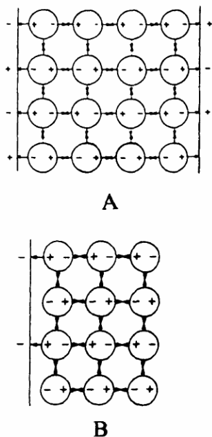
Figure 20. Diagrammatic illustrations of how arrays of alternately positively-, and negatively-charged fixed sites (on a matrix of linear chains [NP-NP-NP system], not shown or) on juxtaposed surfaces (NP-NP system) (A), or of alternately negatively-charged and neutral sites (NO system) (B) can produce the dynamic structure of polarized-oriented multilayers of water molecules. A stable three-dimensional cooperatively-linked assembly of water molecules follow from charge-dipole interactions with the fixed charged sites and from both radial and lateral dipole-dipole interaction with oppositely orientated neighboring water molecules. (From Ling 155 by permission of John Wiley & Sons, Inc.)
