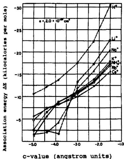
Figure 42. The theoretically computed association-energies in kilogram calories per mole of H^+ , Li^+ , Na^+ , K^+ , Rb^+ , Cs^+ and NH_4^+ respectively on a singly charged oxyacid group with a polarizability of 2.0 \times 10^{-24} \text{ cm}^3 and c -value as indicated on the abscissa. An ion, say K^+ , which shows a higher negative energy of association of -13 \text{ kcal/mole} on the fixed oxyacid anion at a c -value of -4.0 \text{ \AA} is preferentially adsorbed over Na^+ , which at the same c -value, shows a lower negative association energy of -3.5 \text{ Kcal/mole} only. However, at higher c -value of -2.5 \text{ \AA} , the preference is reversed since at this point the negative association energy of Na^+ at -16 \text{ kcal/mole} is higher than that of K^+ at -13 \text{ kcal/mole} . Preference reversal at different c -values is important in physiological activities according to the AI Hypothesis. (From Ling 98 )
