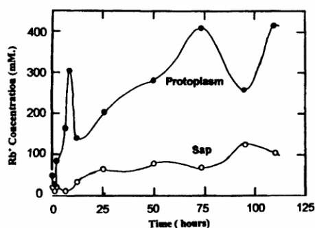
Figure 67. Oscillatory uptake of radioactively labeled \text{Rb}^+ by the protoplasm of Nitella interstitial cells (top curve) and its delayed release (bottom curve) into the (cell) sap in the central vacuole. Experiment lasted 120 hours in water containing 5 mM labeled \text{RbCl} . Each data point represent the mean of 5 determinations in 5 series of studies. pH was 7.3 and the Illumination continuous. (After Brooks 492 )
