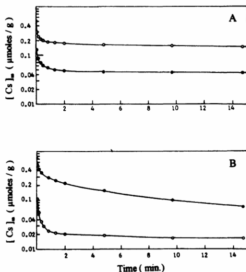
Figure 62. Efflux curves of labeled \text{Cs}^+ from small clusters of frog ovarian eggs. Clusters of frog ovarian eggs were incubated at 25^\circ\text{C} for 4\frac{1}{2} hours in a modified Ringer's solution with or without 10^{-6} M of ouabain. Blotted dry, the egg clusters were incubated at 25^\circ\text{C} for exactly 13 minutes in incubation solution containing 2.0 mM tagged \text{Cs}^+ and 20 mM of competing non-labeled alkali-metal ions. Again blotted dry, the egg clusters were washed in successive portions of non-labeled Ringer's solution. The radioactivity of labeled \text{Cs}^+ detected in the successive portions of washing solution plus the residual labeled \text{Cs}^+ in the egg at the end of the experiment, allow the reconstruction of the efflux curves shown. Control eggs (empty circle); ouabain-treated eggs (solid circles). A, competing ion, \text{Na}^+ . B, competing ion, \text{Rb}^+ . (Ling and Fu 398 )
