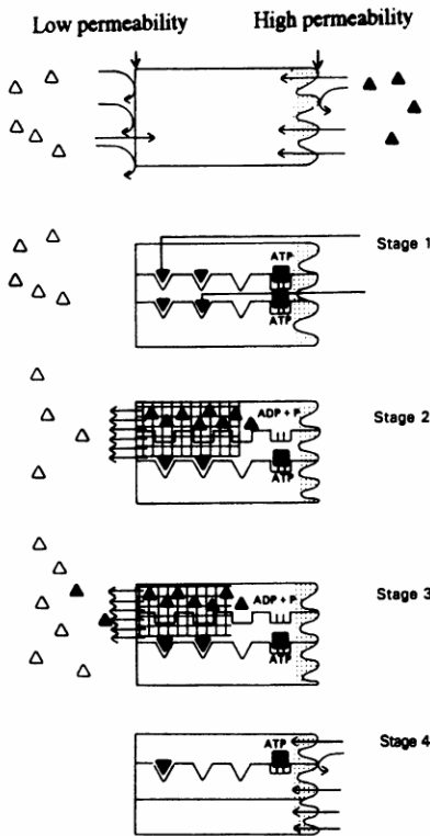
Figure 65. Schematic diagram of the theory of active transport across a bifacial epithelial cell layer. Solute ( \blacktriangle ) from the source aqueous phase in contact with the mucosal surface at right, is transported actively to the sink aqueous phase in contact with the serosal surface at left. \Delta represents the same solute in the sink aqueous phase. Straight and curved arrows indicate respectively successful and unsuccessful attempts at entry. \blacktriangledown represents the solute adsorbed on sites on the sponge protein in the epithelial cells. Clear area in the cell is filled with polarized-oriented multilayers of cell water. Cross-hatched area represents free water. \blacksquare represents ATP which is mostly adsorbed on the protein that possesses Na,K-activated ATPase activity.
