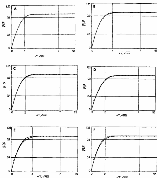
Figure 39. Influx profiles of tritiated water into single frog ovarian eggs (D, E and F) or small clusters of a few eggs (A, B and C). No difference could be detected between these two groups. In all the data obtained, the diffusion is bulk-phase-limited. Solid lines going through or near most data points are theoretical for simple bulk-phase diffusion (A) or for bulk-phase-limited diffusion with adsorption or entry into subcellular compartment (B to F). Dashed lines in B to F are theoretical profiles for simple bulk-phase limited diffusion (as in B of Figure 38) and are included for comparison. The diffusion coefficients obtained from eight sets of studies yield 1.00 \pm 0.10 (S.E.) in units of 10^{-5} \text{ cm}^2/\text{sec} . in comparison with that of tritiated water in normal liquid water at the same temperature ( 25^\circ\text{C} ) equal to 2.44 in the same unit. (Ling et al. 201 reproduced from The Journal of General Physiology by copyright permission of the Rockefeller University Press)
