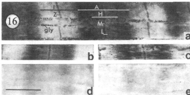
Figure 16. Electron micrographs of dry-cut, unstained section of freeze-dried frog sartorius muscle fibers. Muscles were loaded physiologically with \text{Cs}^+ (a) and \text{Tl}^+ (b,c) before freeze-fixation, freeze-drying and embedding. (c) was obtained after exposure of a cut section to room
