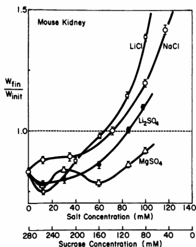
Figure 63. Percentage weight changes as that of initial weights (ordinate) of isolated mouse kidneys in response to chilling (4°C) and anoxia, plotted against the concentrations of salts plus sucrose in the bathing solutions shown on the abscissa. Sucrose is added to maintain a constant isotonic osmolarity. Different salts used are shown against the weight curves of the mouse kidneys incubated in the solution containing that salt-sucrose combination (e.g., 60 mM of NaCl + 160 mM of sucrose). Data show that both Na^+ and Cl^- are essential to produce maximum swelling, but LiCl is even more effective than NaCl . (From Ling and Kwon 199 )
