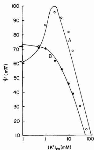
Figure 69. Effect of ouabain ( 10^{-4} M) on the resting potential of "Na-rich" rat soleus muscle. (A) Control Na + -loaded muscle; (B) ouabain-treated Na + -loaded muscle. Na + -loaded soleus muscles were isolated from rats fed a low K + diet. Experimental points are the same as shown in Figure 68 and are taken from Akaike. 240 Their resting potentials were measured in the presence of varying concentrations of external K + with or without ouabain. Both solid lines going through or near most data points are theoretical based on Equation A19. In (A), -\gamma/2 = 0.67 Kcal/mole, K_{Na \rightarrow K}^{oo} = 96.3 , constant_1 = 116 mV. In (B), -\gamma/2 = 0 Kcal/mole, K_{Na \rightarrow K}^{oo} = 35 , constant_1 = 76.4 mV. (From Ling, Baxter and Leitmann 314 )
