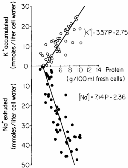
Figure 33. Reuptake of K^+ and extrusion of Na^+ from red-blood-cell “ghosts” prepared from washed human red blood cells. The study followed rigorously a procedure described in Reference 471. Freshly drawn blood was obtained (mostly) from different donors. When blood from the same donors was used, it was drawn at at least 6-weeks intervals. Each data point represents the difference of K^+ or Na^+ concentration in samples of the ghosts at the beginning of incubations and after 18 hours of incubation in the presence of ATP ( 37^\circ\text{C} ). Straight lines corresponding to the two equations shown in the graph were obtained by the method of least squares. Total protein content represented as P in the equations was obtained by subtracting the sum of the weights of lipids, phospholipids, salt ions, and sucrose from the dry weights of the ghosts. (Ling, Zodda and Sellers 140 )
